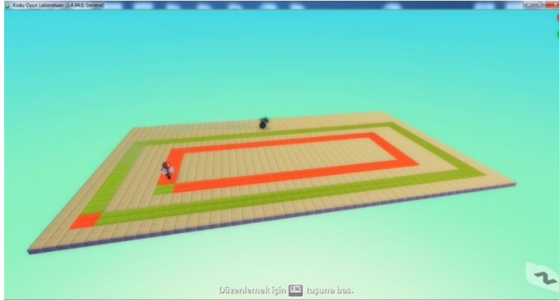
Figure 12. Game screen
